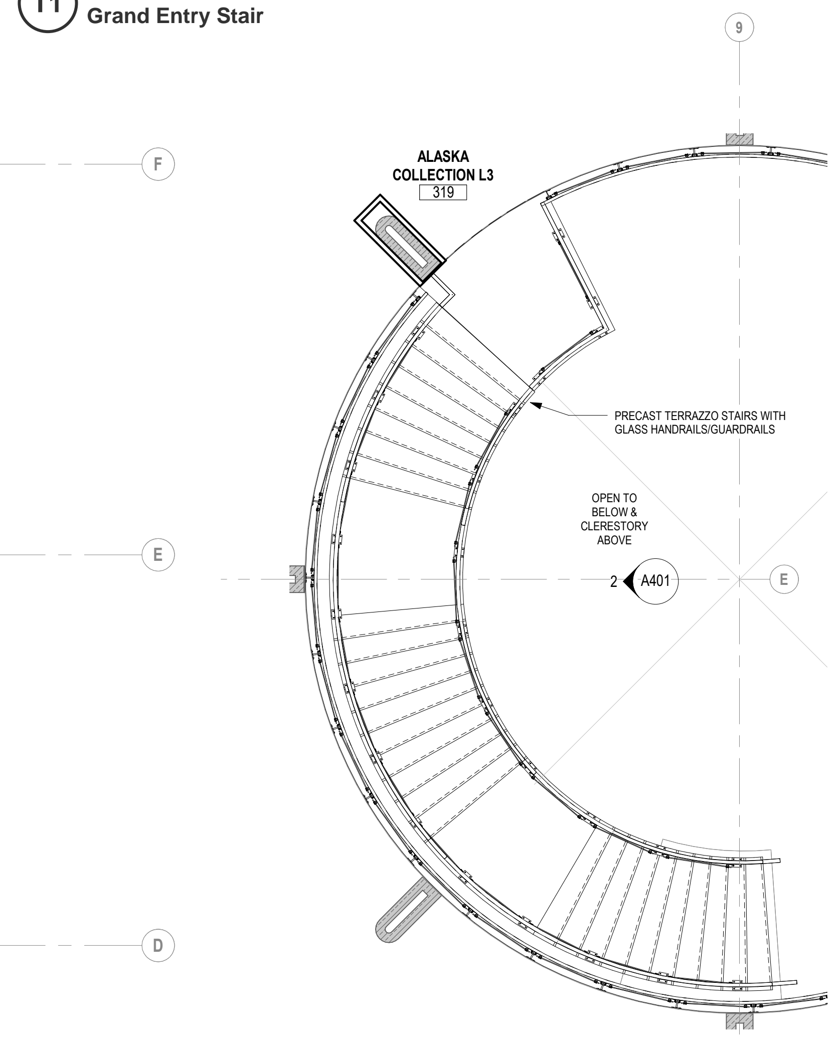
PRECAST TERRAZZO STAIR - AK COLLECTION TO EVENT CENTER
